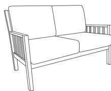
LOUNGE 2 128 x 90 x 78 cm Back cushion 2x (60 x 46 x 13 cm) Seat cushion 2x (60 x 66 x 17 cm)
