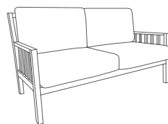
LOUNGE 2,5 158 x 90 x 78 cm Back cushion 2x (76 x 46 x 13 cm) Seat cushion 2x (76 x 66 x 17 cm)
